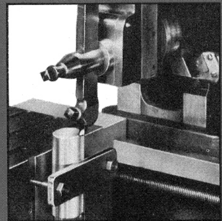
Machining end of round piece of work held in "V" groove on side of table.
